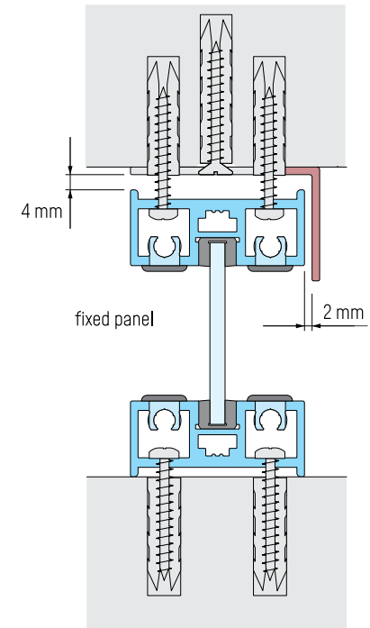
FIXED PANEL
