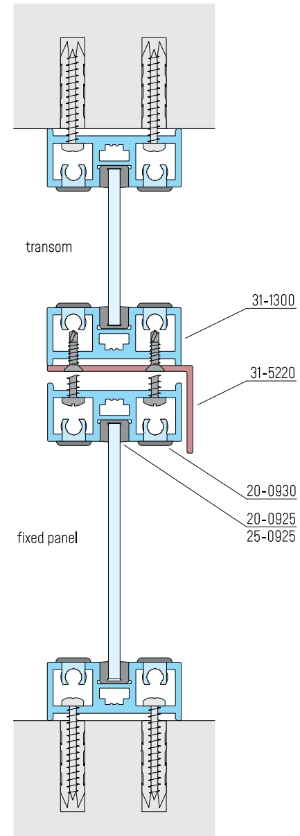
TRANSOM WITH FIXED PANEL
