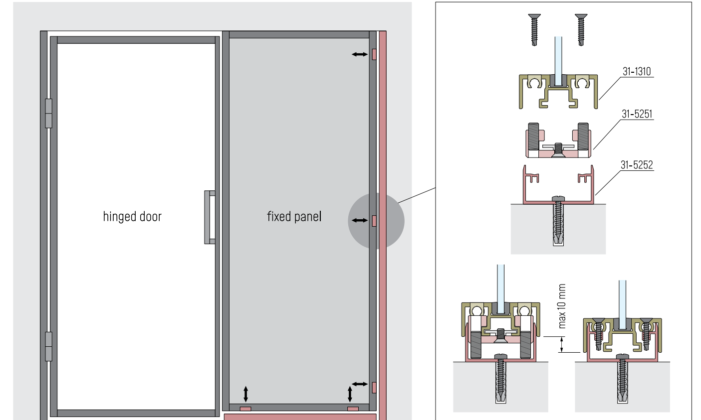
FIXED PANEL ADJUSTMENT OPTION
