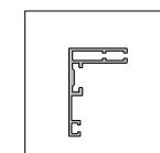
31-1603 AL31 DOOR FRAME CASING 30, 5300 MM AN, CM
