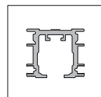
27-2110 AL27-2 TOP TRACK 2, 5000 MM
