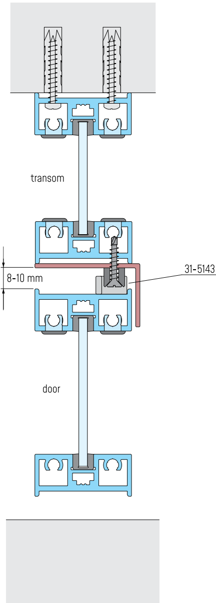
TRANSOM WITH HINGED DOORS
