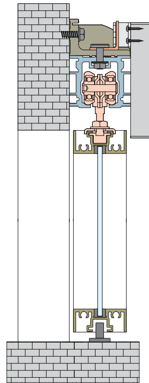
FIXED TO THE WALL
