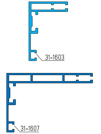
FRAME ASSEMBLING
