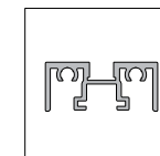
31-1310 AL31 OPEN RAIL 3050MM AN, CM
