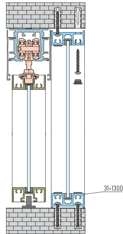
SLIDING DOOR AND FIXED PANEL
