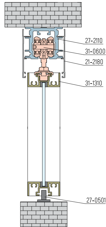
FIXED TO THE CEILING
